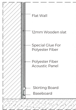
Polyester Fiber Acoustic Panel Wall Installation(Paste Direct)
