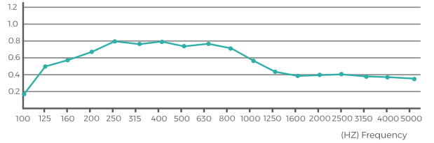
Sound absorption coefficient
