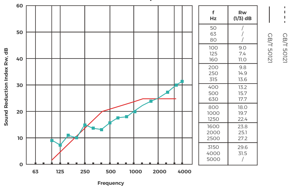
Sound Reduction Data Curve Graph
