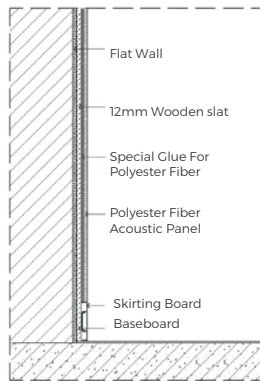
Polyester Fiber Acoustic Panel Wall Installation(Paste Directly)
